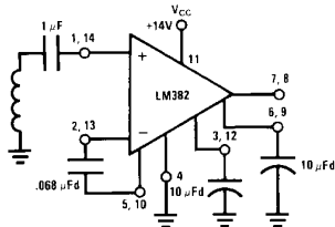
Tape Preamp (NAB Equalization)
