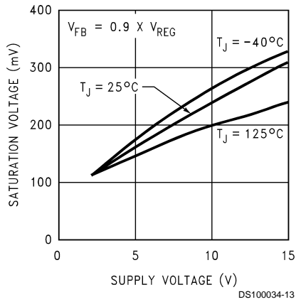
Gate-Ground Saturation
