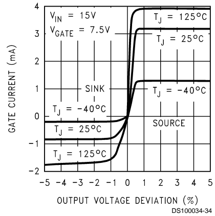
Gate Current
