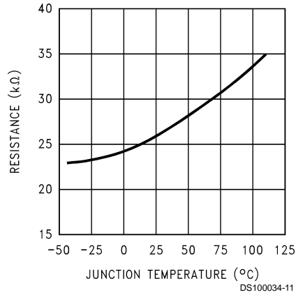
ON/OFF Input Resistance
