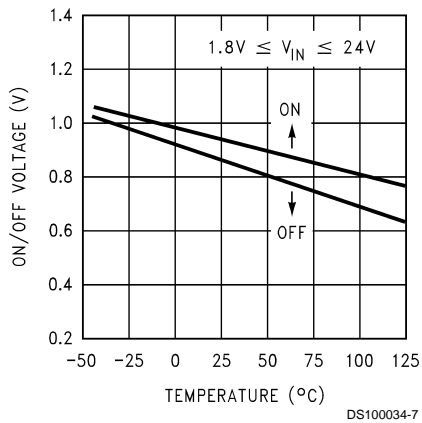
ON/OFF Threshold
