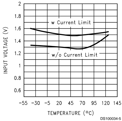
Minimum Operating Voltage
