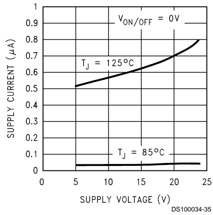
Leakage Current
