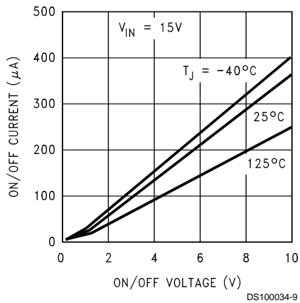
ON/OFF Pin Current
