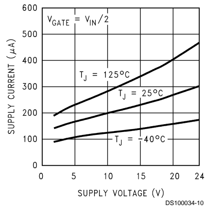
Supply Current
