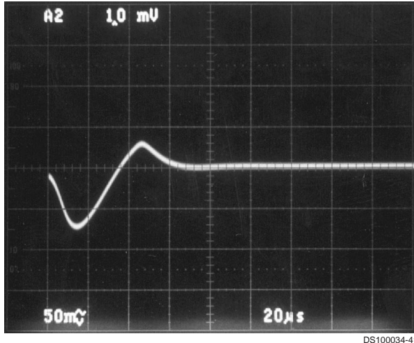
Transient Response for 0–6A Load Step
