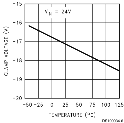
V_{IN} Referred Gate Clamp Voltage
