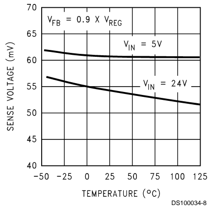
Current Limit Sense Voltage
