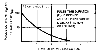
FIGURE 2 PULSE WAVEFORM FOR EXPONENTIAL SURGE
