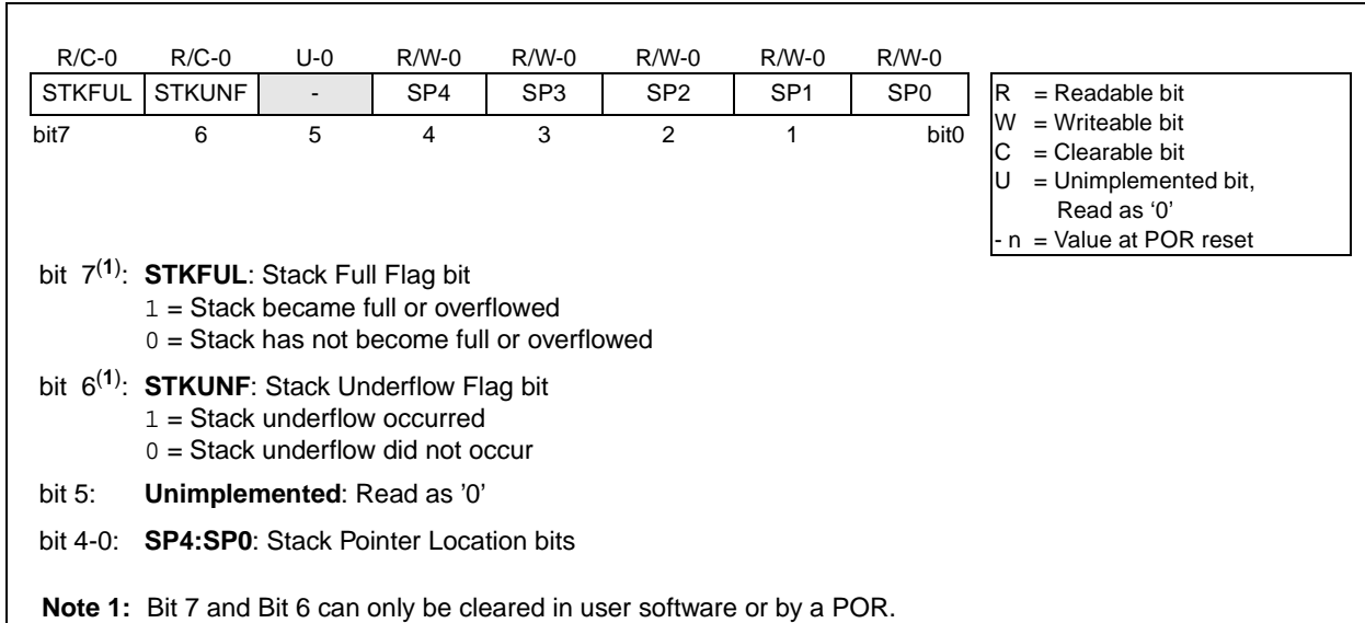
Register 4-1: STKPTR - Stack Pointer Register
